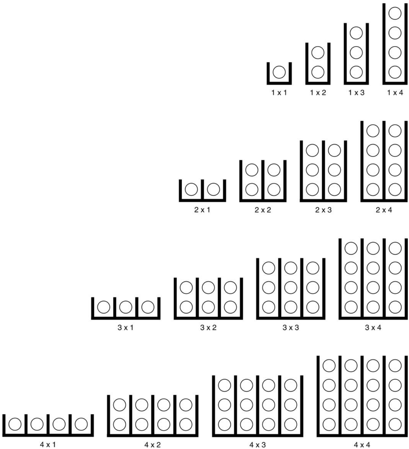
Cylinder Barricade Racks Overhead view showing cylinder placement
